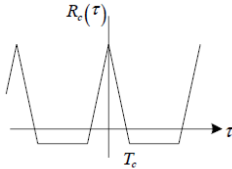
Fig. 1. Autocorrelation of PN sequence
