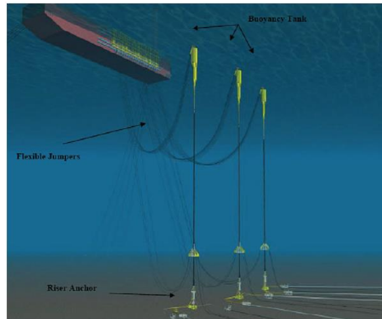
Figure 26-6 Bundled Hybrid Riser Diagram
