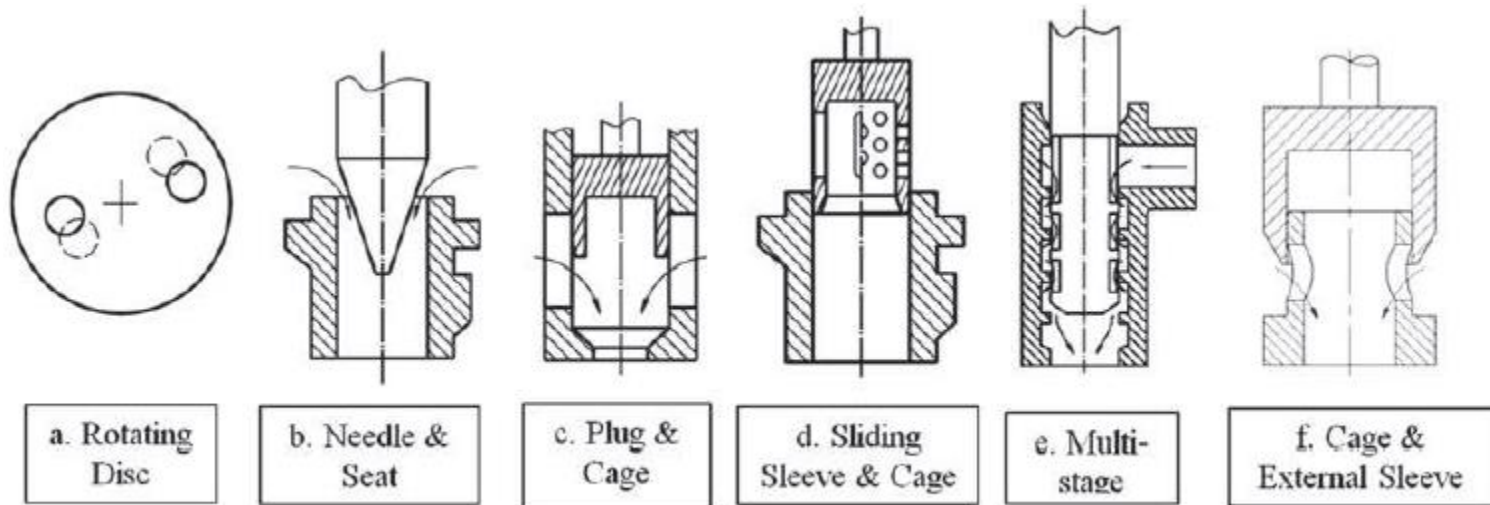
Figure 22-32 Trim Types
