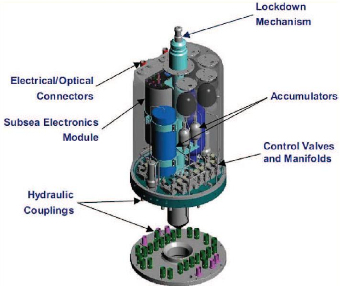
Figure 22-37 SCM Configuration
