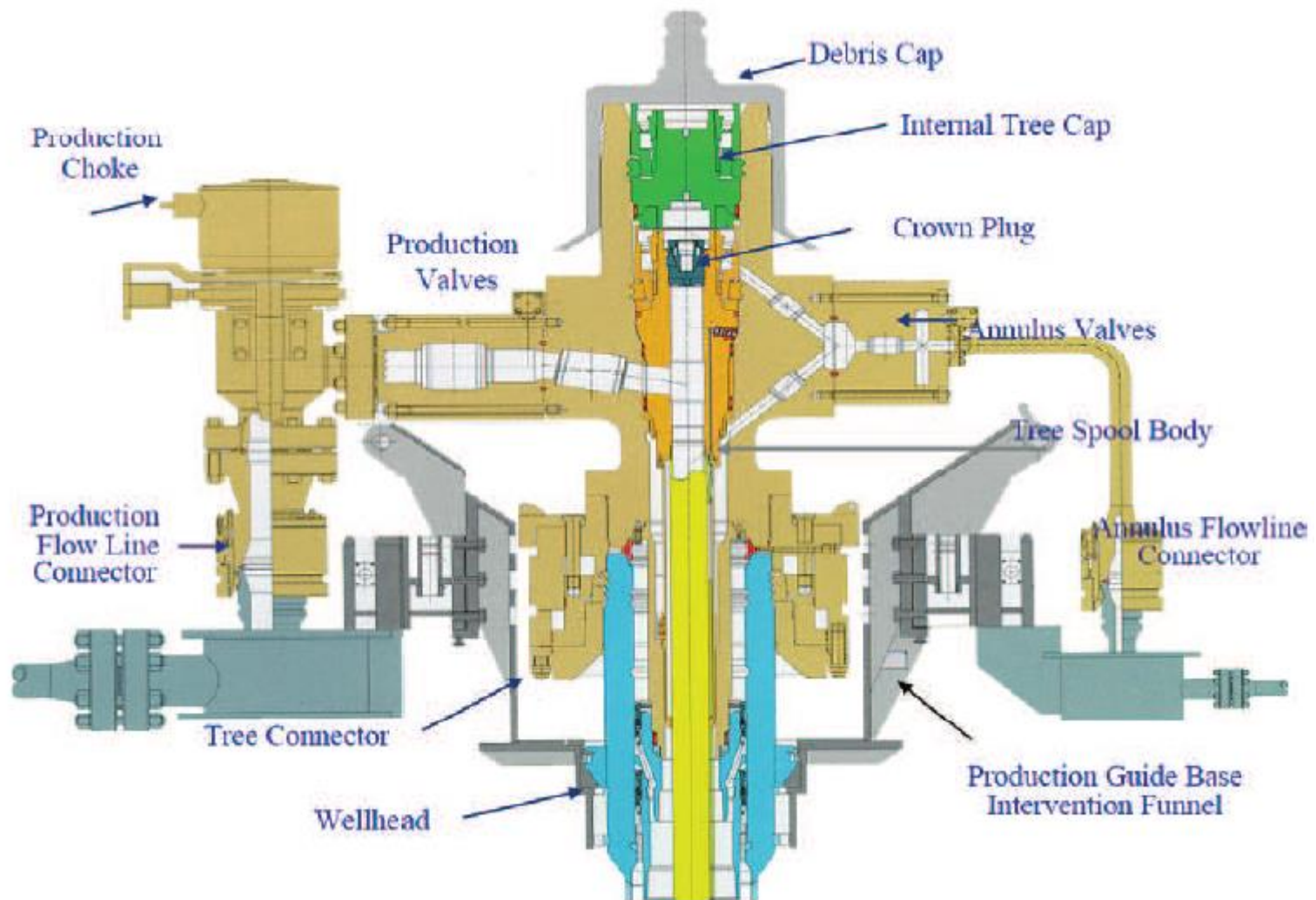
Figure 22-22 Typical Components of an HXT
