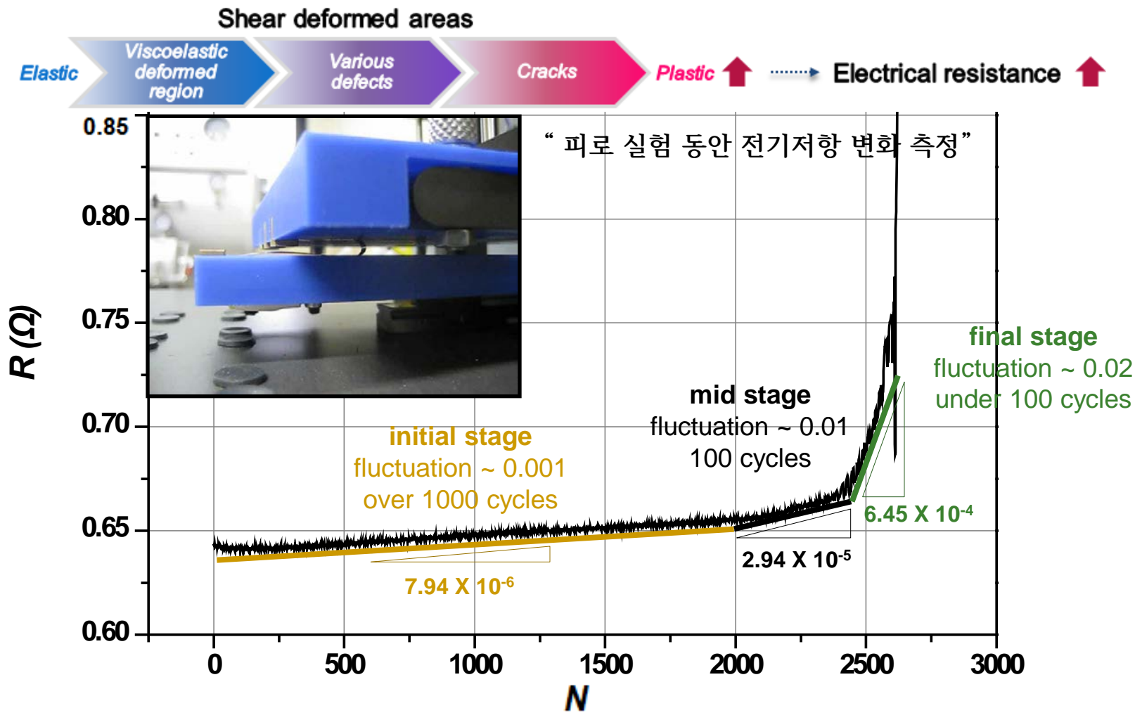
Measurement of resistance change during bending fatigue test of MG ribbons
