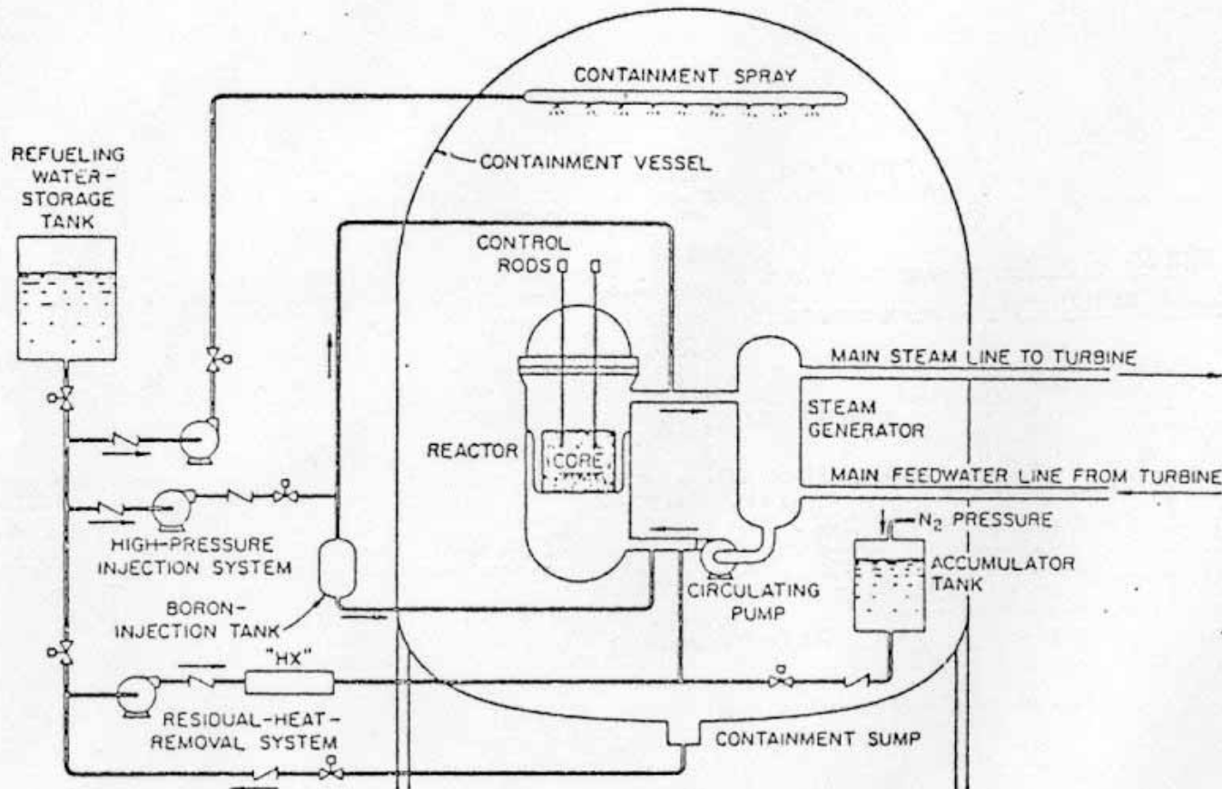
Fig. 1 PWR emergency core-cooling system.
