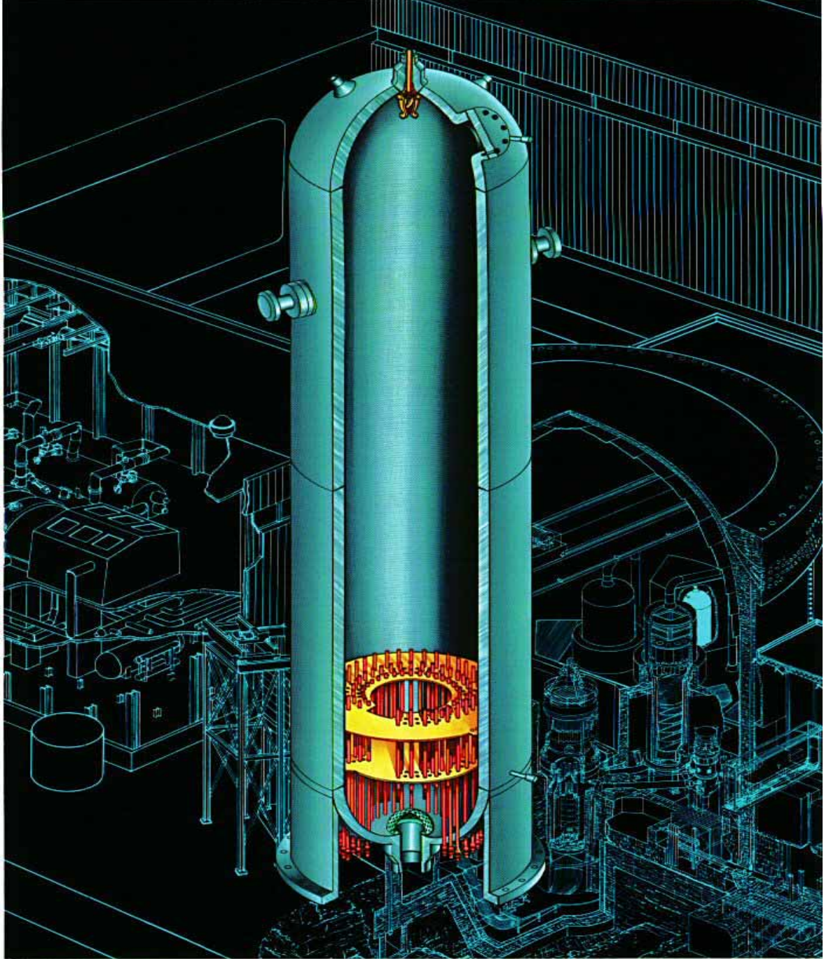
Westinghouse PRESSURIZER
