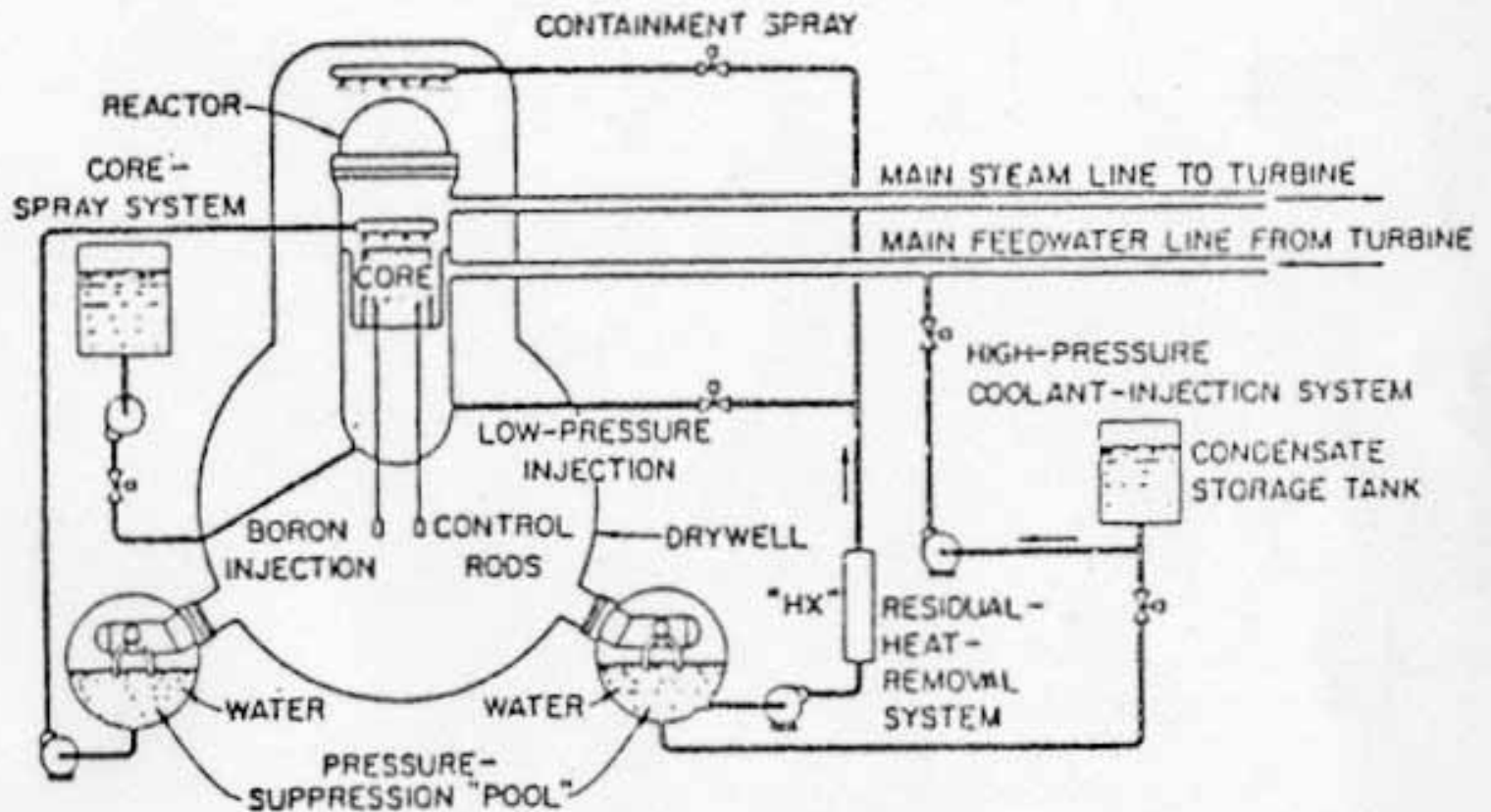
Fig. 2 BWR emergency core-cooling system.
