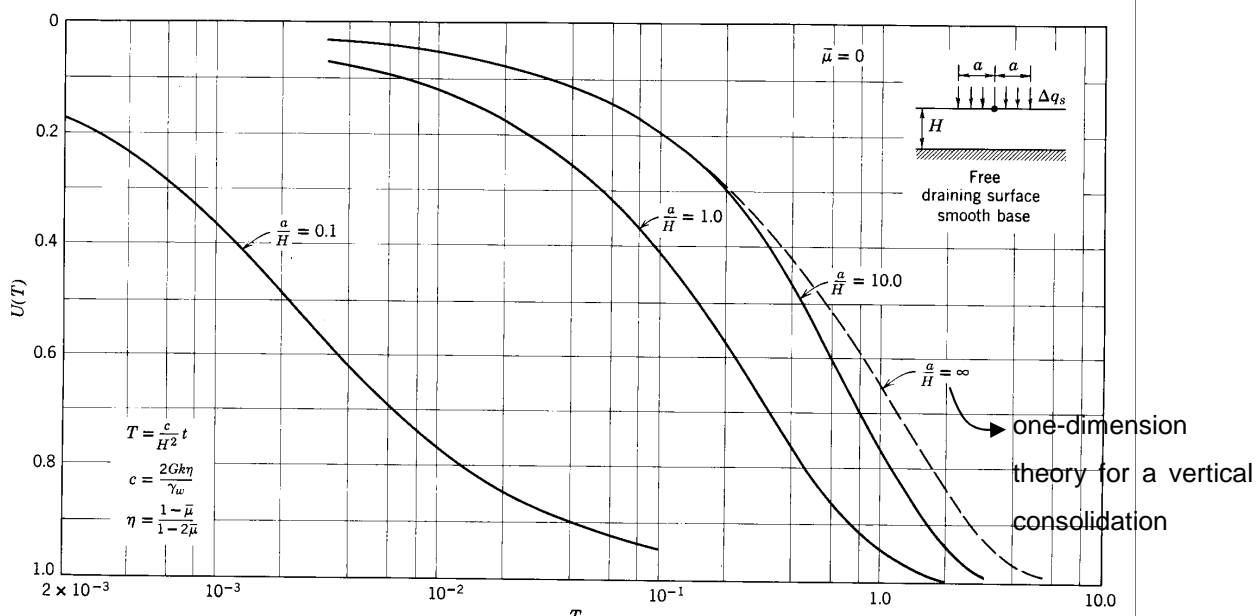
Fig. 2-56 Consolidation of stratum under circular load (From Gibson, Schiffman, and Pu, 1967).
