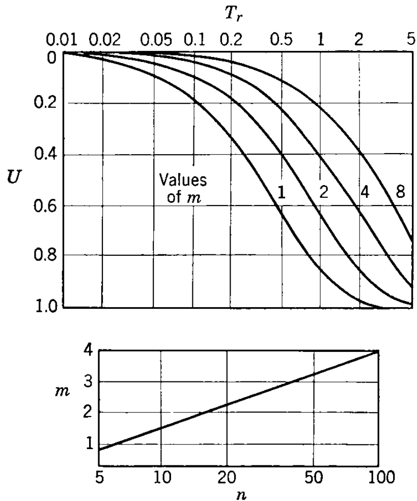
Fig. 2-58 Average consolidation ratio for radial drainage by vertical drains (After Scott, 1963)
