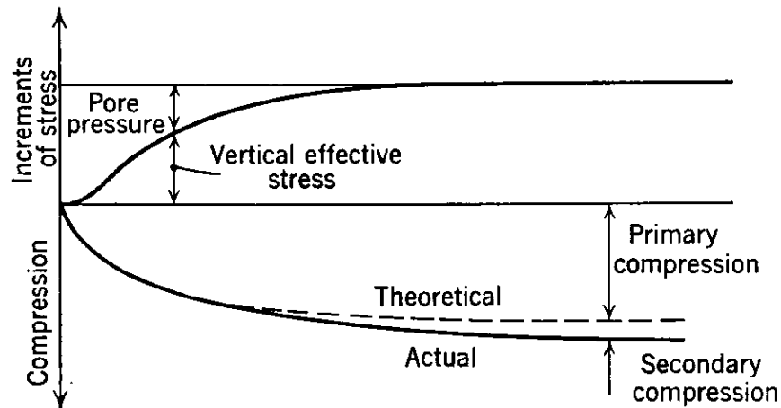
Fig. 2-59 Primary and secondary compression
