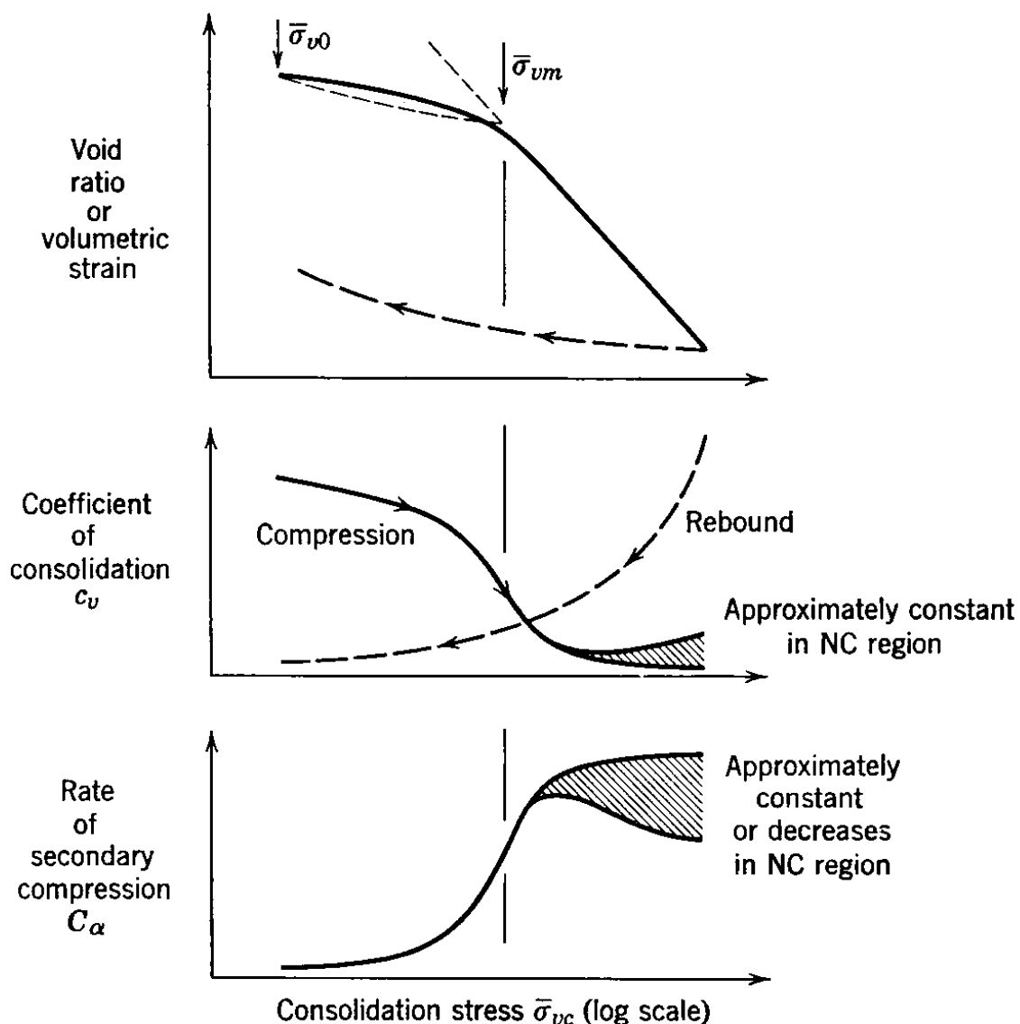
Fig. 2-50 Typical variation in coefficient of consolidation and rate of secondary compression with consolidation stress.
