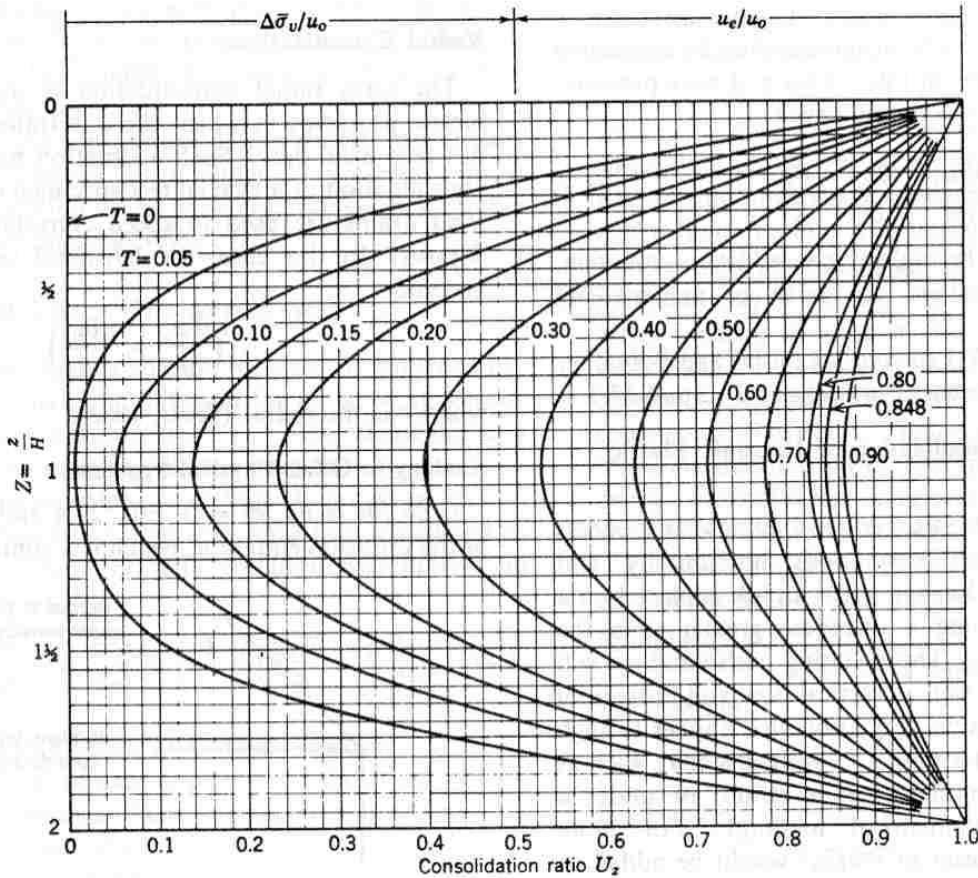
Fig. 2-47 Consolidation ratio as function of depth and time factor: uniform initial excess pore pressure.
