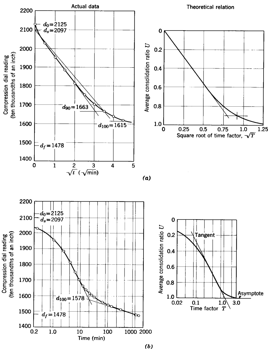
Fig. 2-49 Time-compression compression curves from laboratory tests. Analyzed for c_v by two methods. (a) Square root of time fitting method. (b) Log time fitting method. (From Taylor, 1948.)
