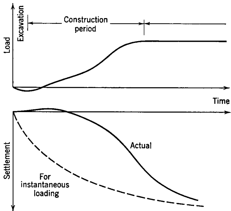
Fig. 2-52 Settlement from time-varying load.
