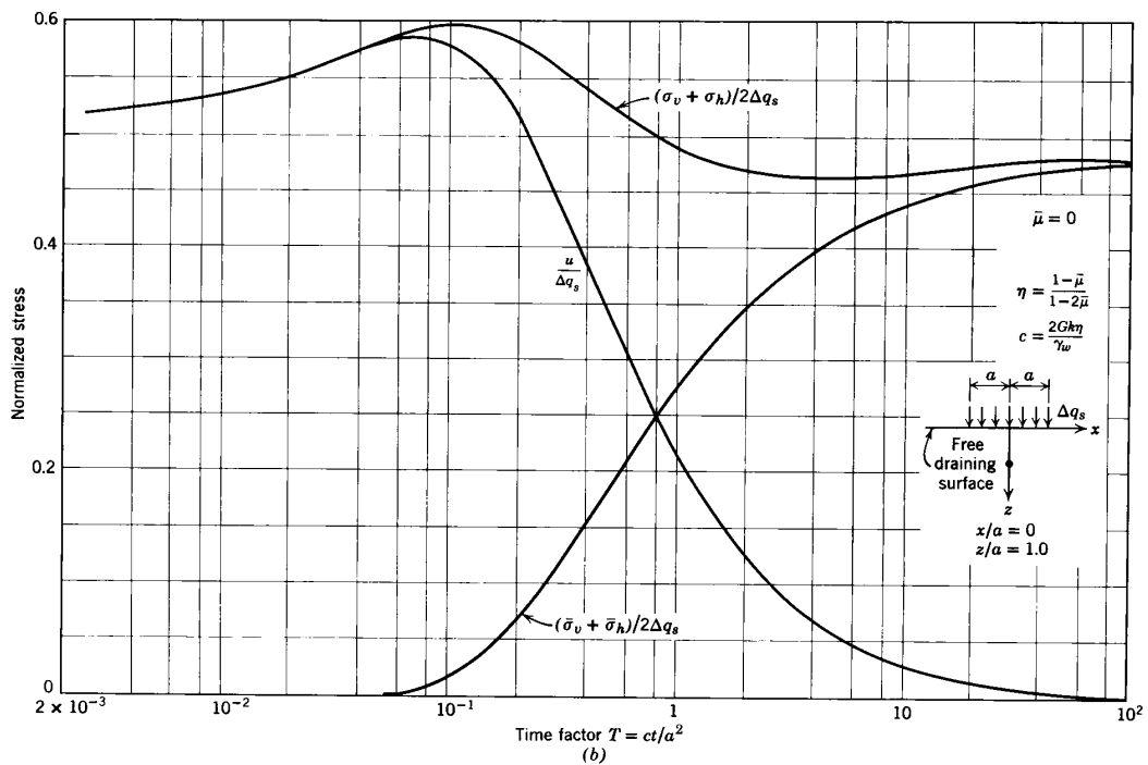
Fig. 2-55 Two-dimensional consolidation beneath a strip load. (From Schiffman et al., 1967).
