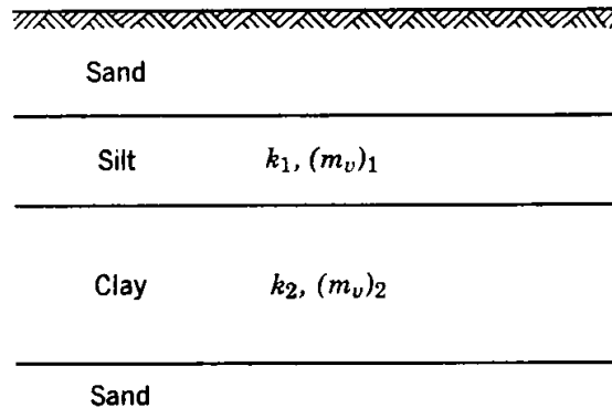
Fig. 2-53 Consolidation problem with two compressible strata.
