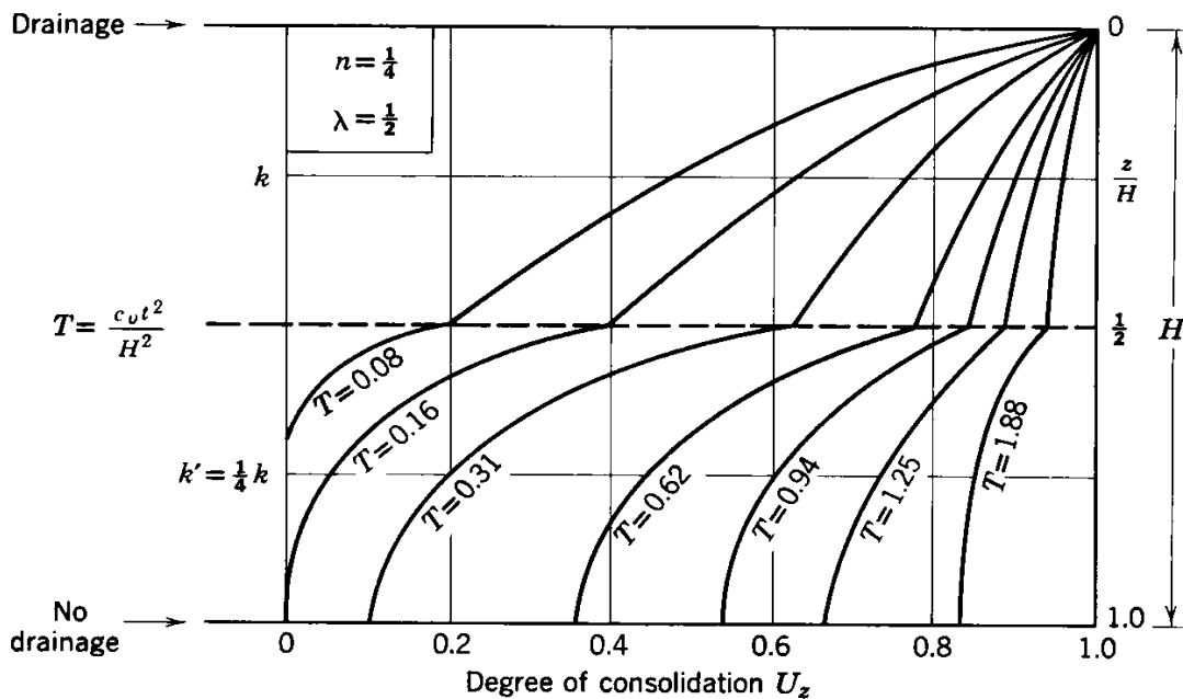
Fig. 2-54 Consolidation of two layers. C_v and k for bottom layer are 1/4 of values for upper layer. T is based upon C_v of upper layer (from Luscher, 1965).
