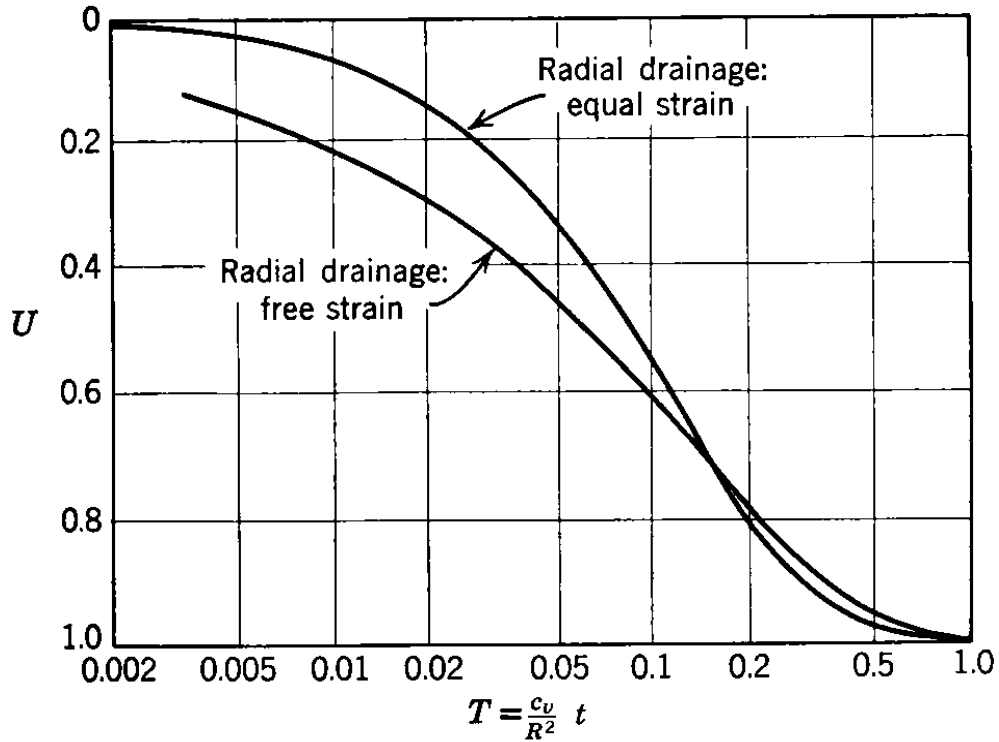
Fig. 2-57 Average consolidation ratio for radial drainage in triaxial test (After Scott, 1963).
