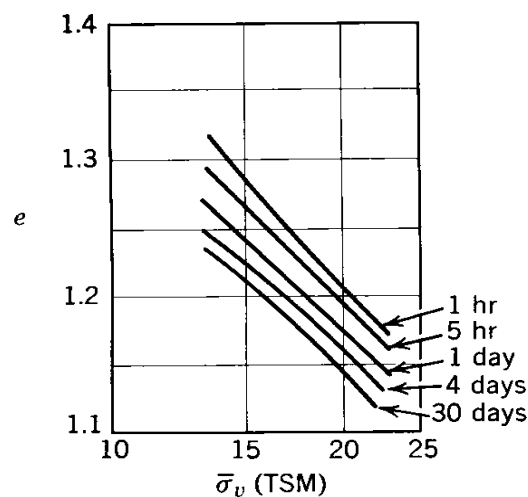
Fig. 2-60 e versus \log \bar{\sigma}_v as function of duration of secondary compression (After Bjerrum, 1967)
