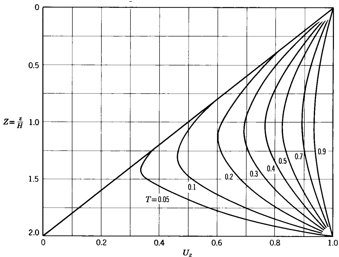
Fig. 2-51 U_z versus Z for triangular initial excess pore pressure distribution. (Upside down of Fig 2-39)
