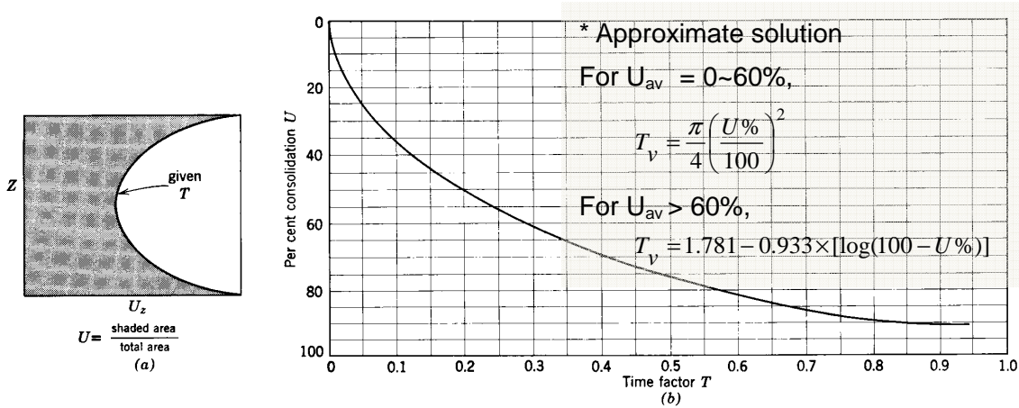
Fig. 2-48 Average consolidation ratio : linear initial excess pore pressure.
