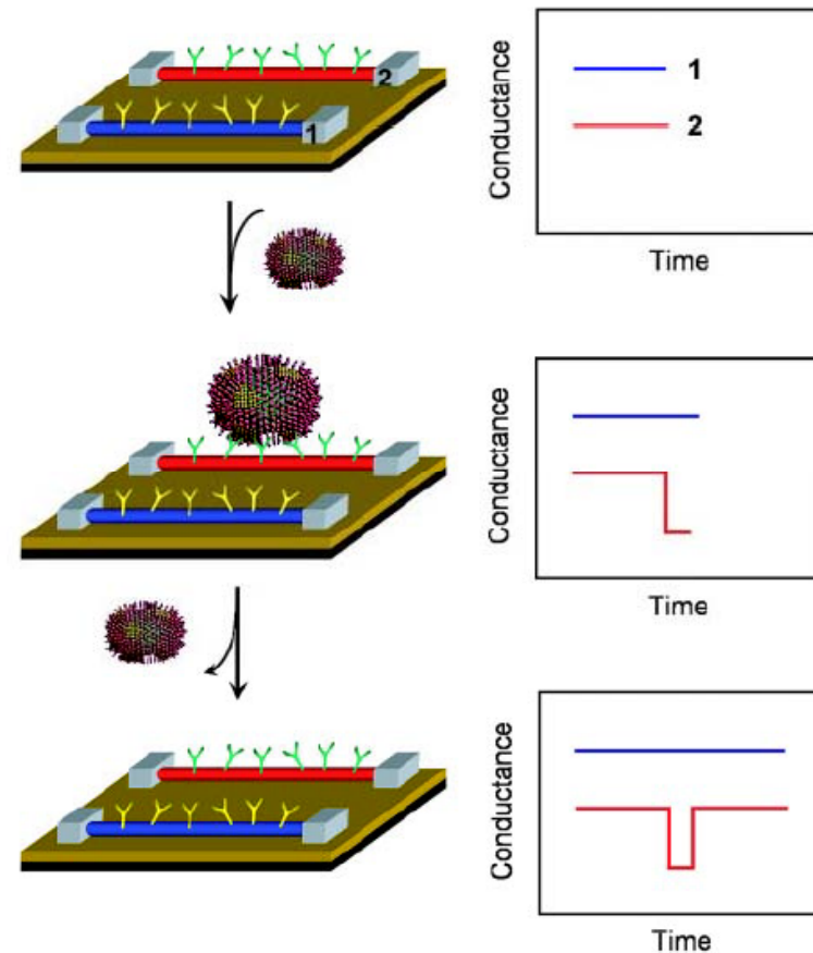
Fig. 1. Nanowire-based detection of single viruses. ( Left ) Schematic shows two nanowire devices, 1 and 2, where the nanowires are modified with different antibody receptors. Specific binding of a single virus to the receptors on nanowire 2 produces a conductance change ( Right ) characteristic of the surface charge of the virus only in nanowire 2. When the virus unbinds from the surface the conductance returns to the baseline value.
