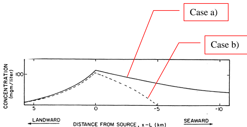
Figure 7.24 Longitudinal concentration distributions for Example 7.5: — discharge 30 km from the mouth; --- discharge 5 km from the mouth.
