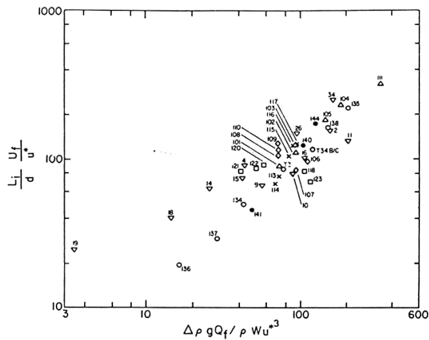
Figure 7.13 A correlation of observed salinity intrusions in laboratory flume experiments. Numbers beside points are run numbers given in the references. \nabla Ippen and Harleman (1961); other data from Rigger (1973) using one base condition and varying one parameter at a time identified as follows: \circ tidal amplitude, \times channel roughness, \triangle channel length, \square fresh water discharge, \diamond mean depth, \bullet ocean salinity.
