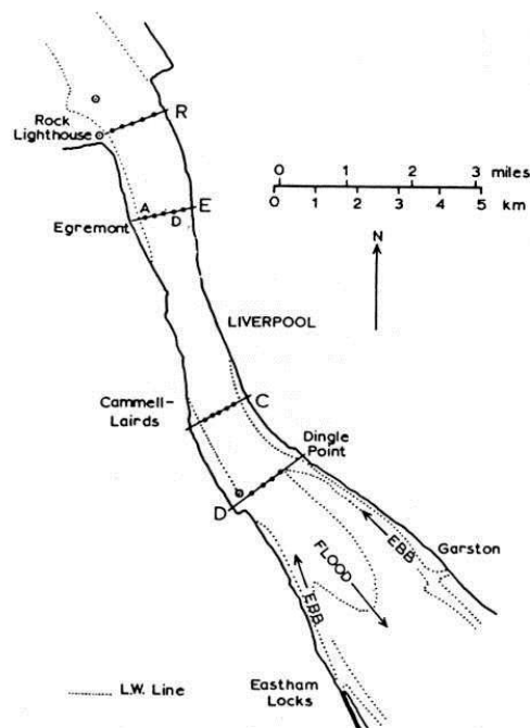
Figure 7.5 The narrows of the Mersey estuary, England. Dotted lines represent the low water line; arrows show the flood and ebb channels. [After Bowden and Gilligan (1971).]
