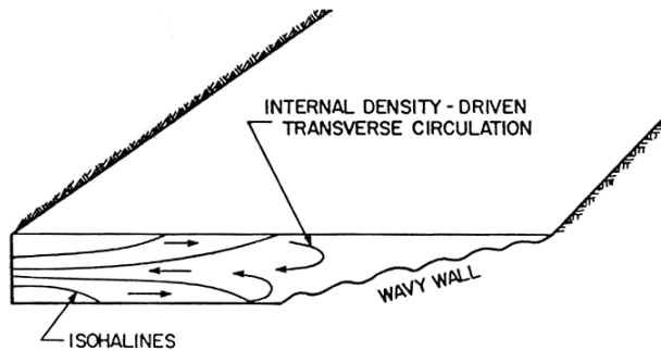
Figure 7.14 A typical distribution of isohalines and the inferred internal density-driven circulation in a channel with one wavy side.
