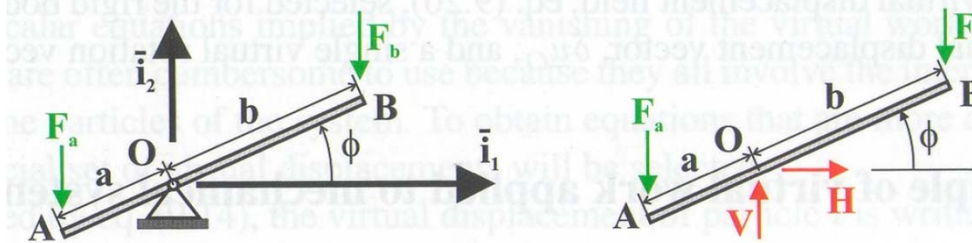
Fig. 9.9. Simple lever acted upon by two vertical end forces.
