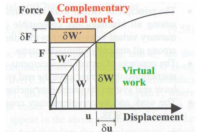
Fig. 9.38. Work and complementary work and their virtual counterparts.
