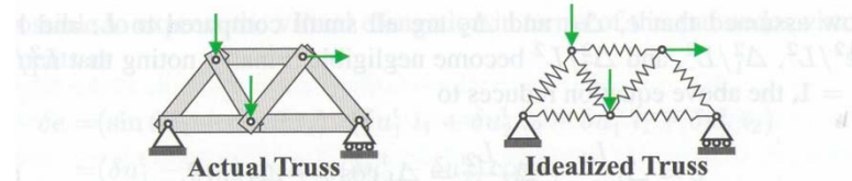
Fig. 9.28. Planar truss and its idealization as an assembly of rectilinear springs.
