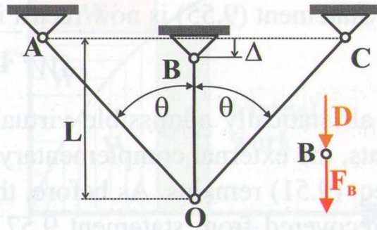
Fig. 9.37. Three-bar truss with prescribed displacement.
