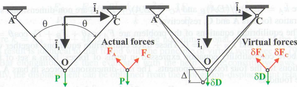
Fig. 9.40. The unit load method for a two-bar truss.
