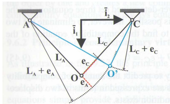
Fig. 9.34. Two-bar truss in the original and deformed configurations.
