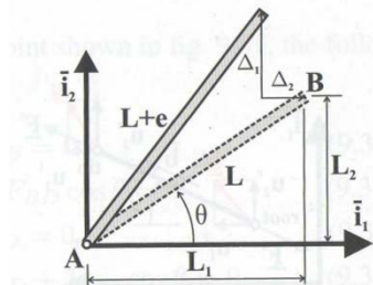
Fig. 9.29. Single bar of a planar truss.
