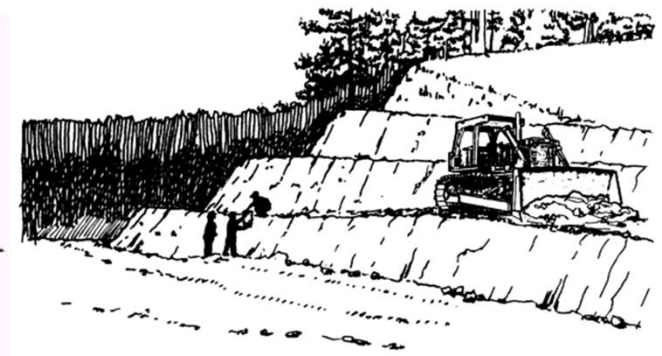
Figure 8-2. Side-hill terracing
