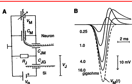
Fig. 4. Circuit of the neuron-Si junction. (A) The circuit consists of the capacitances C_{JM} and C_{JG} , characterizing the plasma membrane and the gate oxide in the junction, and of the resistance R_J characterizing the cleft between membrane and gate. The Si is kept at a voltage V_B . A variable voltage V_M (action potential) is applied across the capacitance C_M of the plasma membrane. The voltage V_J is detected by the source-drain current. (B) Simulation: A pulse V_M(t) of Gaussian shape (amplitude, 40 \text{ mV} ; half width, 2 \text{ ms} ) is applied (dashed line). The voltage V_J(t) is plotted for a junction with C_{JM} = 0.6 \text{ pF} , C_{JG} = 0.1 \text{ pF} , and R_J = 0.25, 1, 4, \text{ and } 16 \text{ gigaohms} . In the case of high resistance, the signal is transmitted efficiently at invariant shape; in the case of low resistance, the signal is differentiated and damped.
