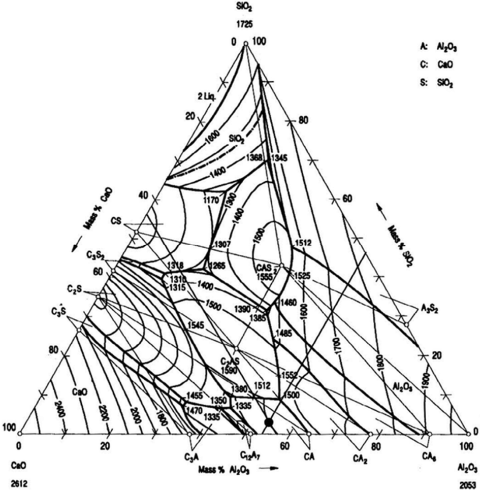
Polythermal projection of CaO-SiO 2 -Al 2 O 3 system
