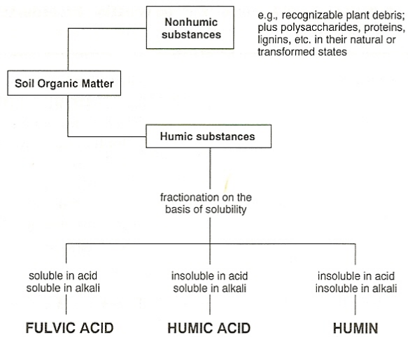
FIGURE 3.4. Fractionation of soil organic matter and humic substances. From Hayes, M. H. B. and Swift, R. S. In "The Chemistry of Soil Constituents" (D. J. Greenland and M. H. B. Hayes, eds.), pp. 179–230. Copyright 1978 John Wiley & Sons, Inc. Reprinted by permission of John Wiley & Sons, Inc.
