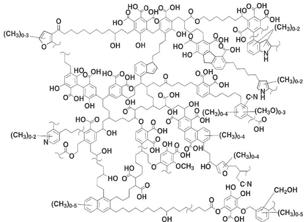
FIGURE 3.5. Schematic of humic acid structure. From Schulten and Schnitzer (1993), with permission from Springer-Verlag.
