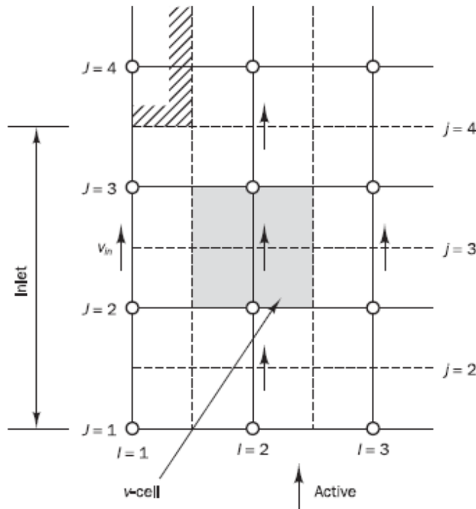
Figure 9.3 v -velocity cell at the inlet boundary
