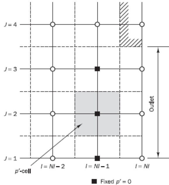
Figure 9.15 p' -cell at an outlet boundary
