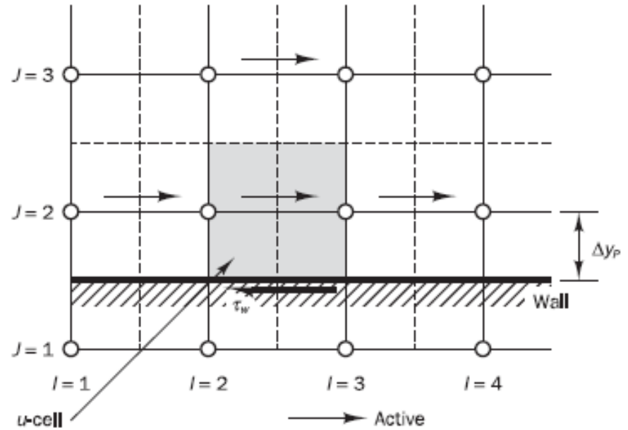
Figure 9.10 u -velocity cell at a wall boundary
