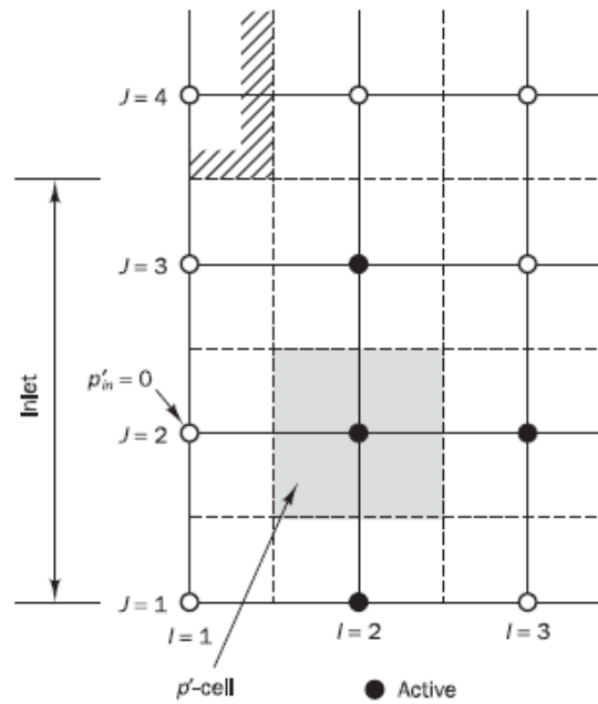
Figure 9.4 Pressure correction cell at the inlet boundary
