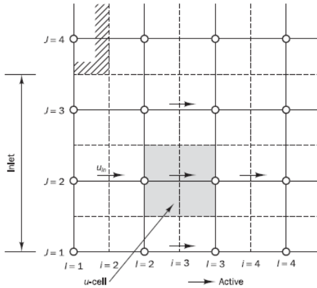
Figure 9.2 u -velocity cell at the inlet boundary
