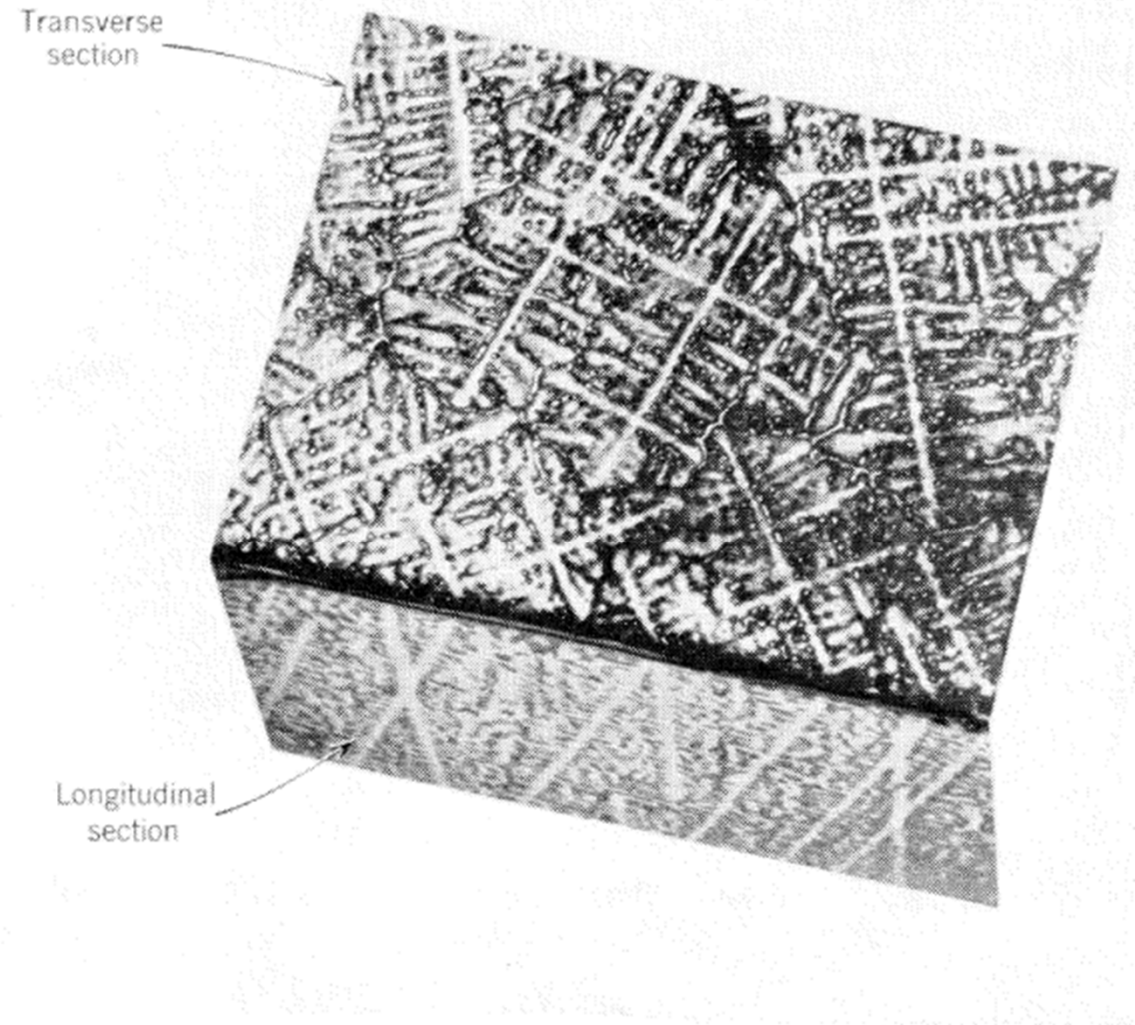
Fig. 5.38. Cellular-dendritic structure.
