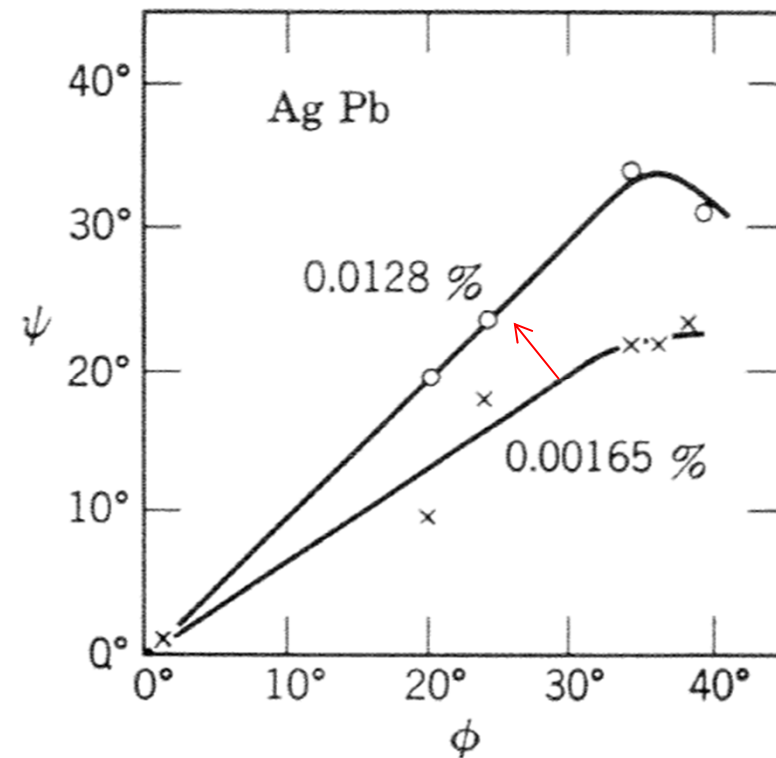
Fig. 5.34. deviation of cellular direction \psi as a function of R (Interface velocity) , dendrite orientation \Phi , and solute content.
