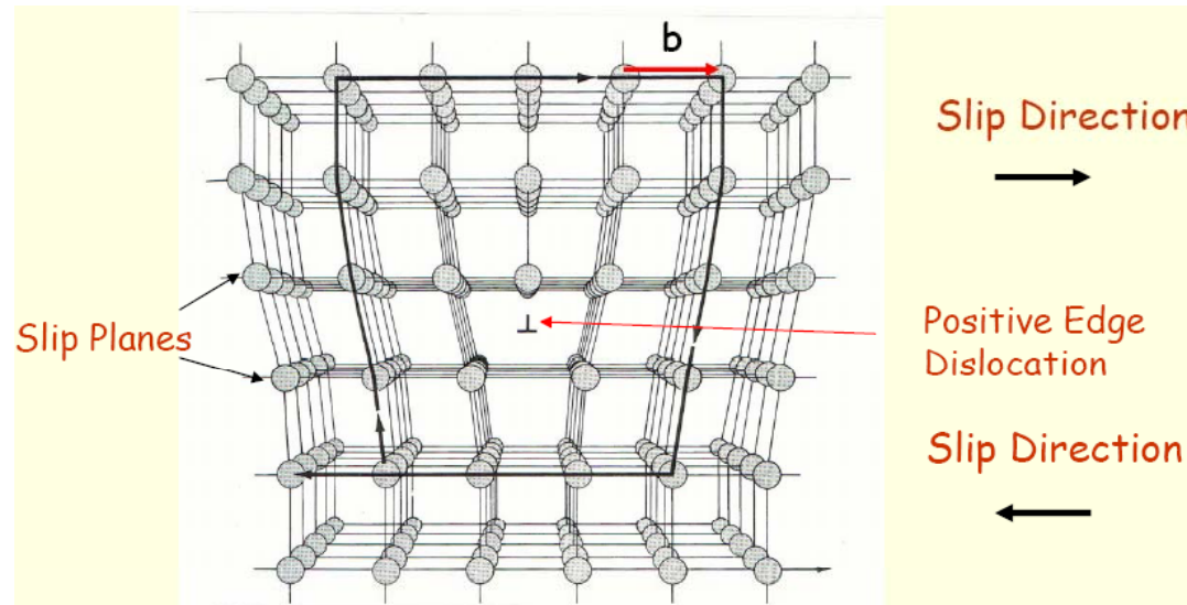
Dislocation (전위)
