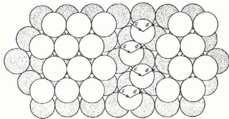
Dislocation (전위)
