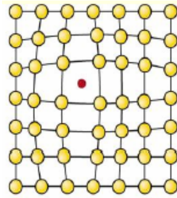
Interstitial 결함
