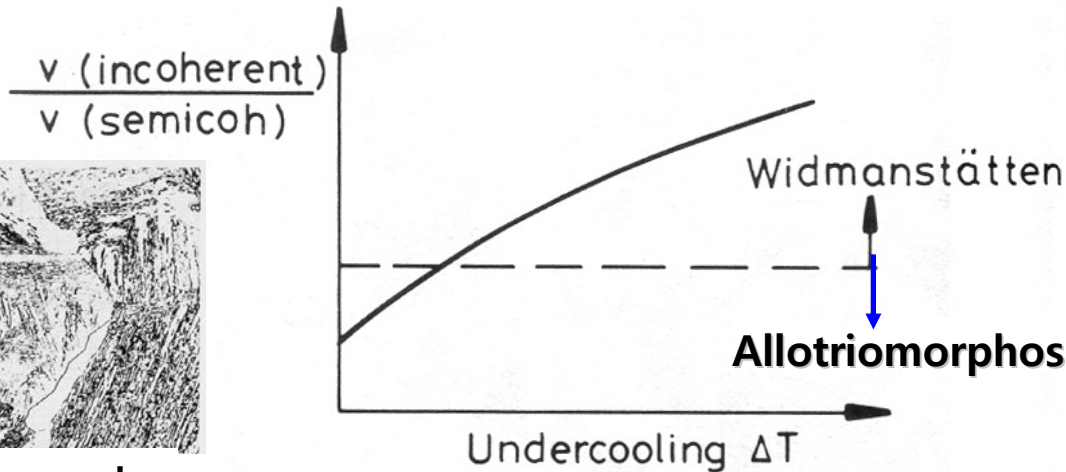
GB allotriomorphs
