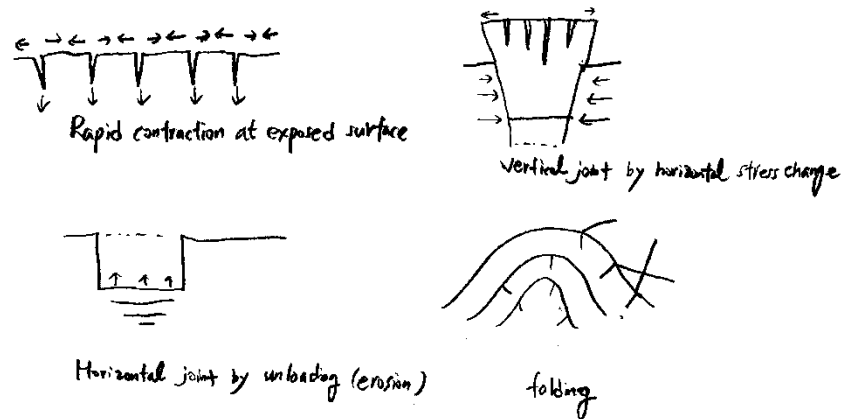
Analysis of rock mass discontinuities
