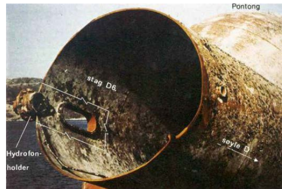
Fig.1.10 Alexander L Kielland accident
