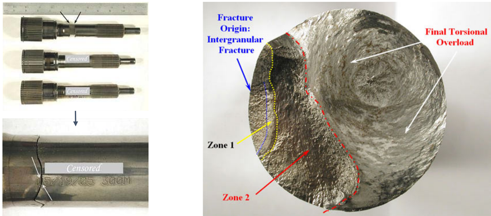
Fig.1.7 Example of fatigue failure (right : Enlargement of the region indicated by white arrow in left-below figure)
