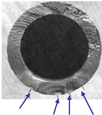
Fig.3.2 Fatigue Surface of Axle Housing
