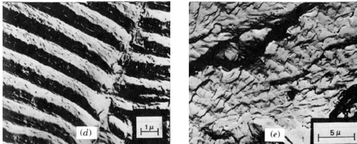
Fig.3.7 Striation (ductile, brittle)
