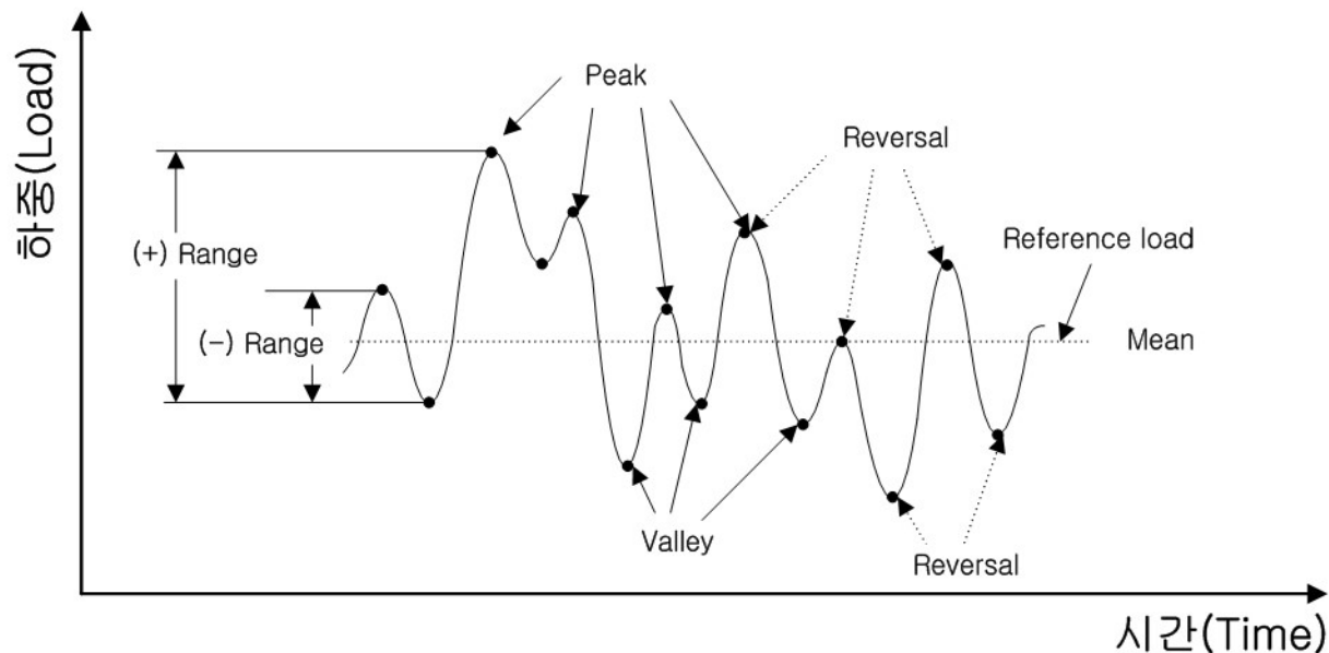
Fig.2.4 Variable loading
