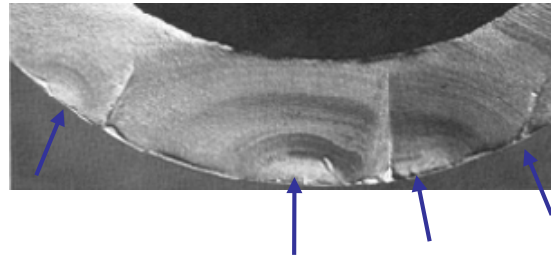
Fig.3.2 Fatigue Surface of Axle Housing
