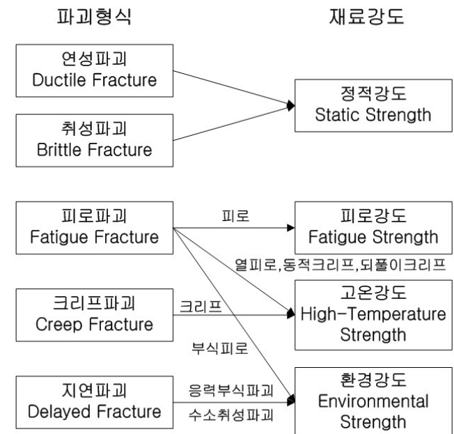
Fig.1.6 Fracture and material strength
