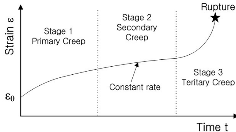
Fig.1.5 Creep deformation
