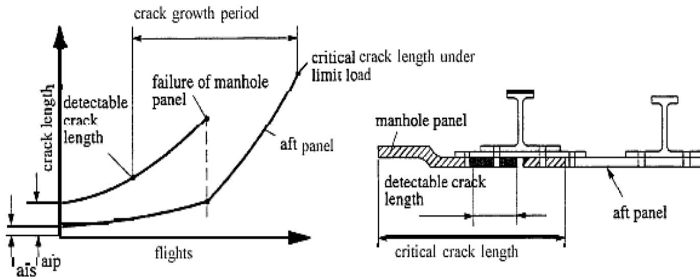
Fig.4.5 Fail-safe design concept (multiple-load path, inspectable for less than one complete load path failure)
