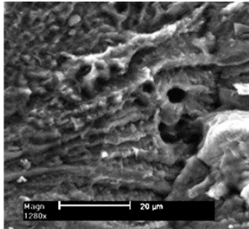
Fig.3.10 Brittle Striation, Aluminum 7075-T6
