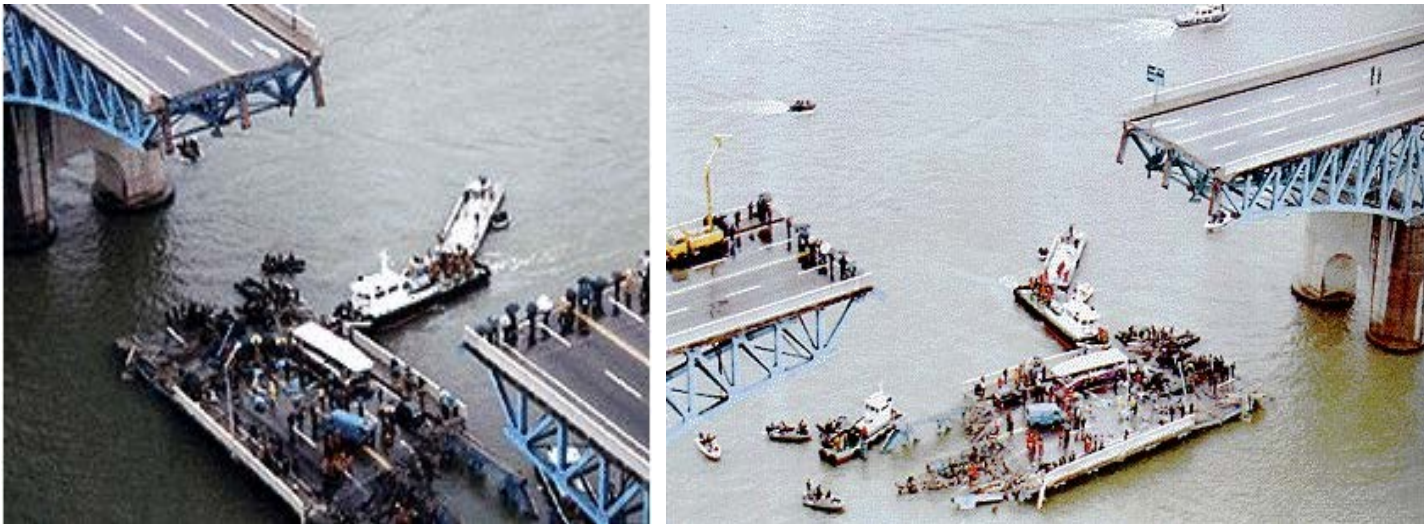
Fig.1.12 Collapses of the Sung Soo Bridge
