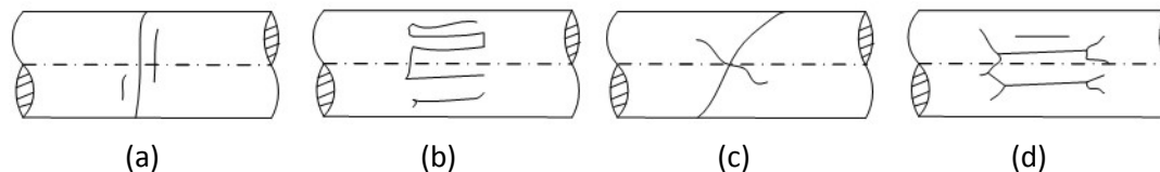
Fig.3.4 Crack configuration of material without notch under torsion
