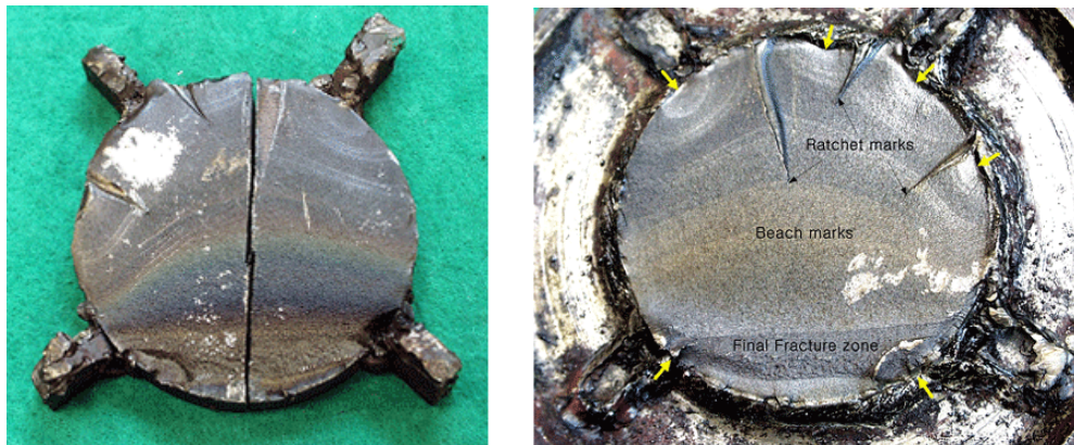
Fig.3.1 Fatigue Surface of Charge Roller
