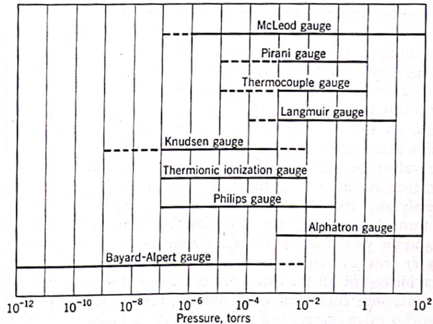
Operating range for various vacuum gauges
