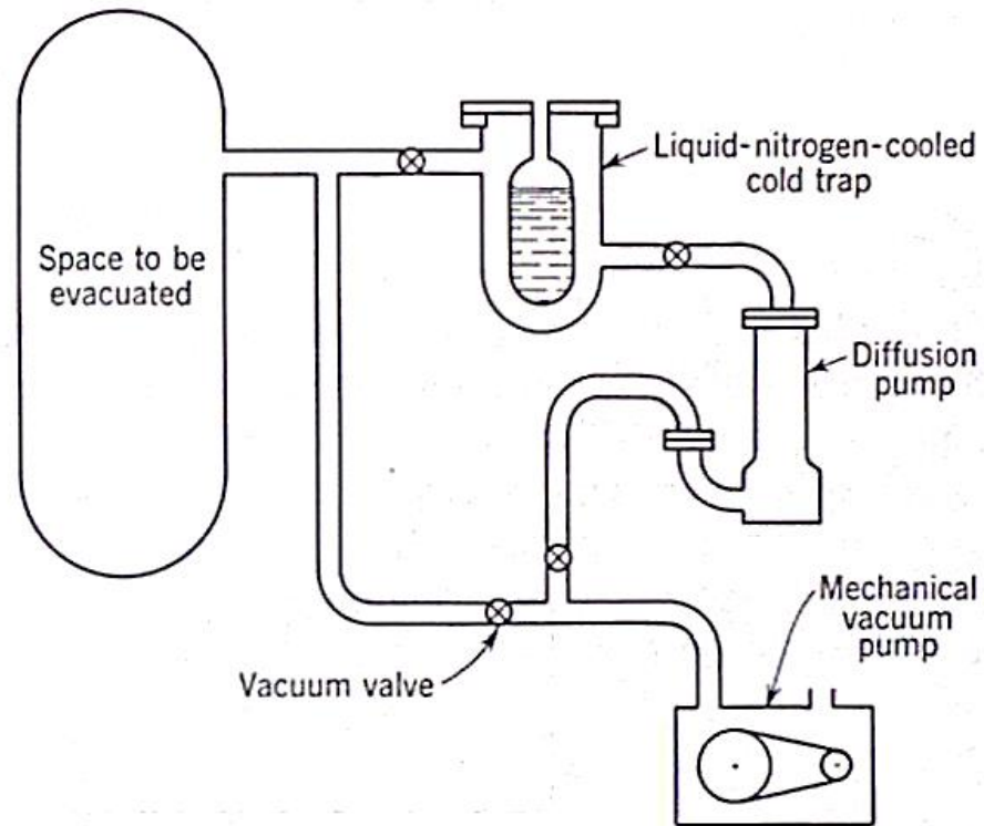
Basic elements of a typical vacuum system
