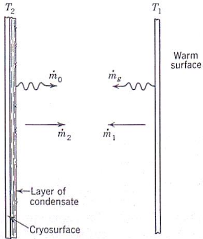
Parallel-plate cryopump system
