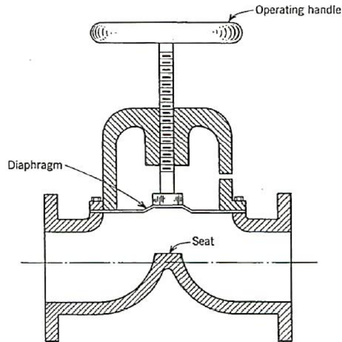
Diaphragm valve
