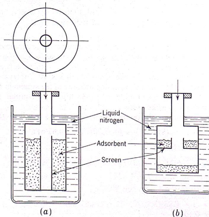
Typical sorption pumps
