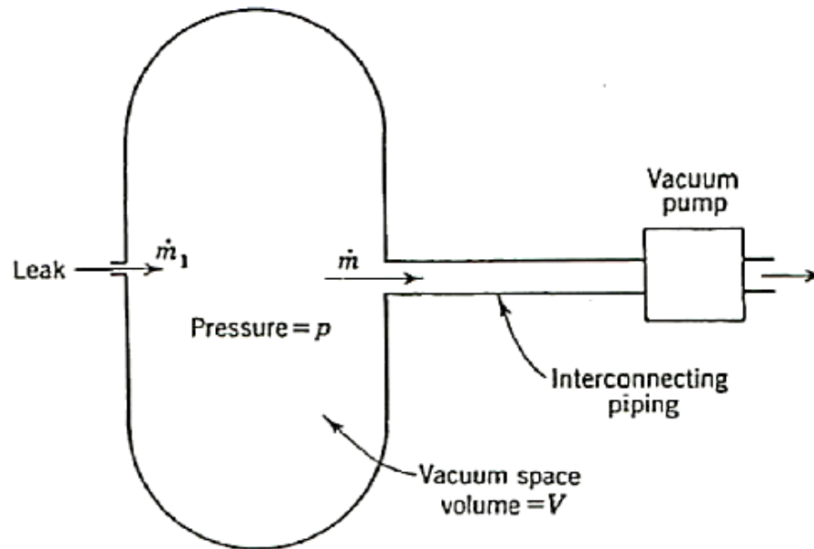
Vacuum system for pump-down equation development
