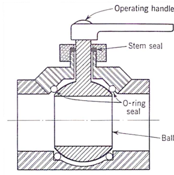
Ball valve
