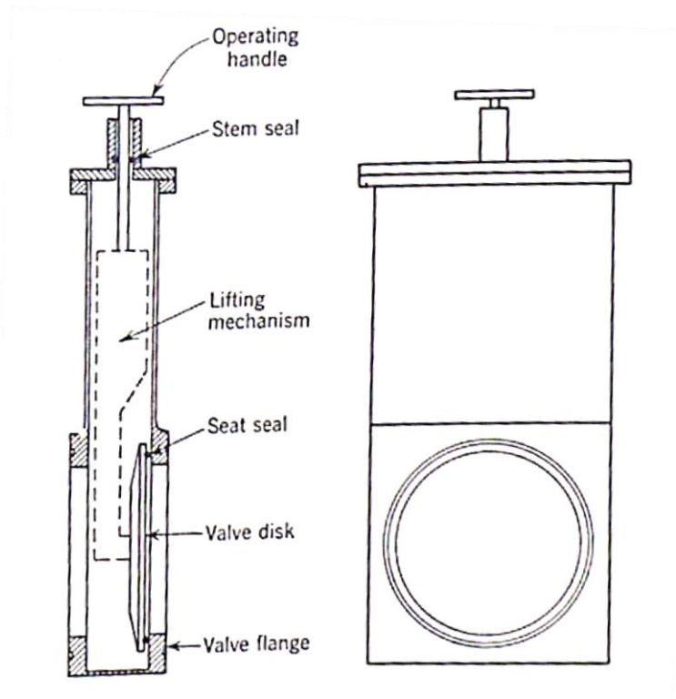
Slide valve for high-vacuum service
