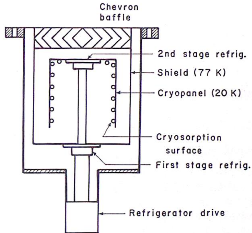
Schematic of a cryosorption pump
