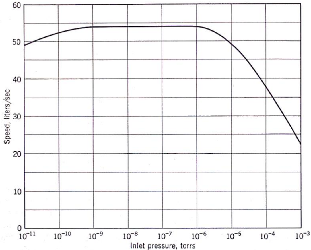
Pumping-speed curve for an ion pump
