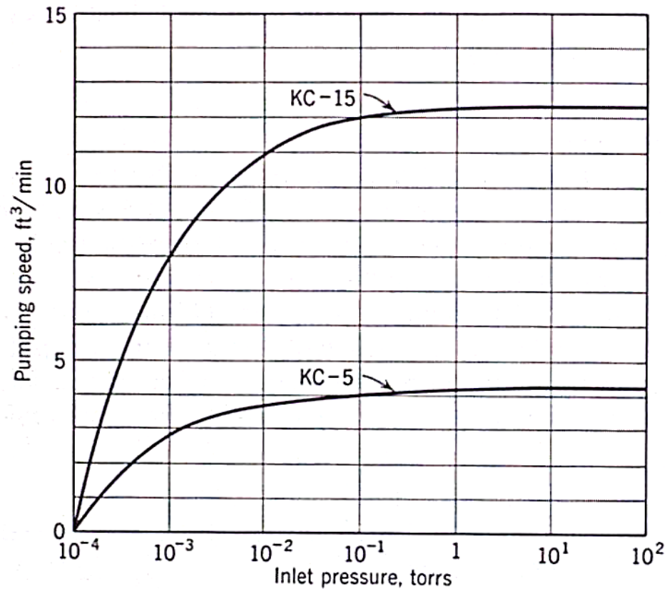
Pumping speed curves for mechanical vacuum pumps
