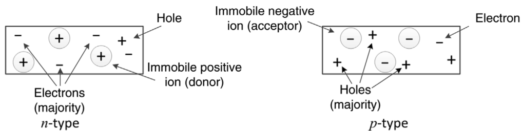
Figure 15.7 Carriers and immobile ions in extrinsic semiconductors.
