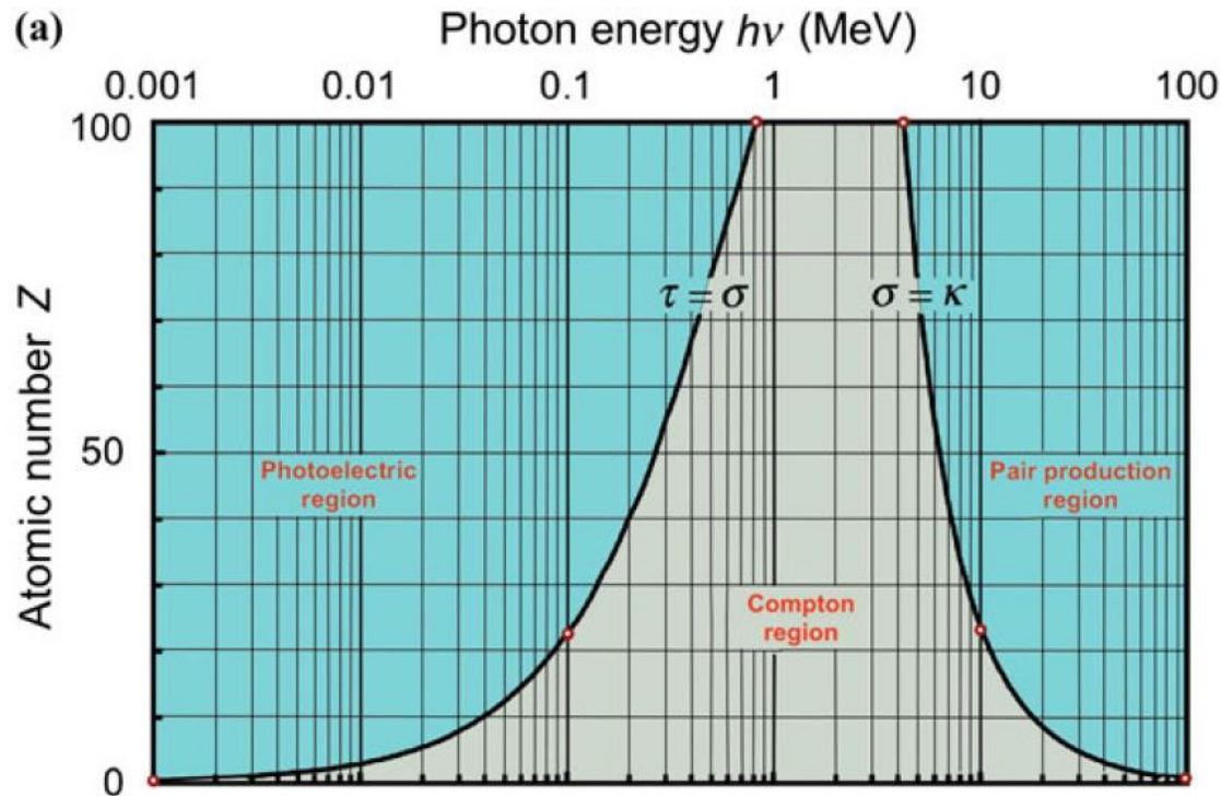
Fig. 8.5 Representation of the relative predominance of the three main processes of photon interaction with absorber atom: photoelectric effect \tau , Compton effect \sigma_C , and pair production \kappa in a (h\nu, Z) diagram where h\nu is photon energy and Z is the absorber atomic number. The two curves in a connect points where photoelectric and Compton cross sections are equal ( \tau = \sigma_C ) shown by the curve on the left and Compton and pair production cross sections are equal ( \sigma_C = \kappa ) shown by the curve on the right . Anchor points for the two curves are: h\nu = 0.001 MeV, Z \approx 0 ; h\nu = 0.1 MeV, Z = 22 ; 0.8 MeV, 100 ; 4 MeV, 100 ; 10 MeV, 22 ; and 100 MeV, 0 . In b we connect specific points
