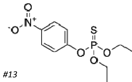
parathion
