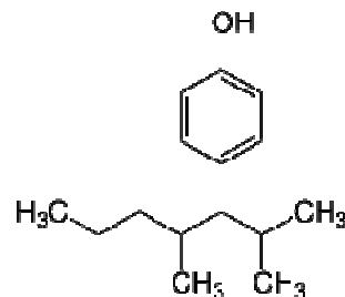
nonylphenol
