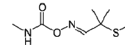
aldicarb
