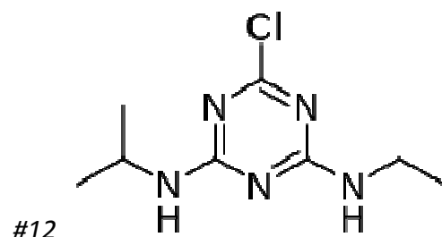
Atrazine
